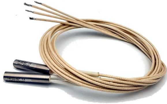
Figure 1 left: NEO9XXHT sensor with 8mm holes for heating cartridges Figure 1 right: NEO20X heating cartridges
