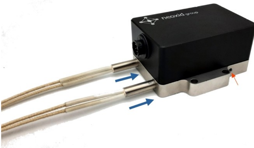
Figure 2: NEO9XXHT sensor with semi-inserted NEO203 heating cartridges
