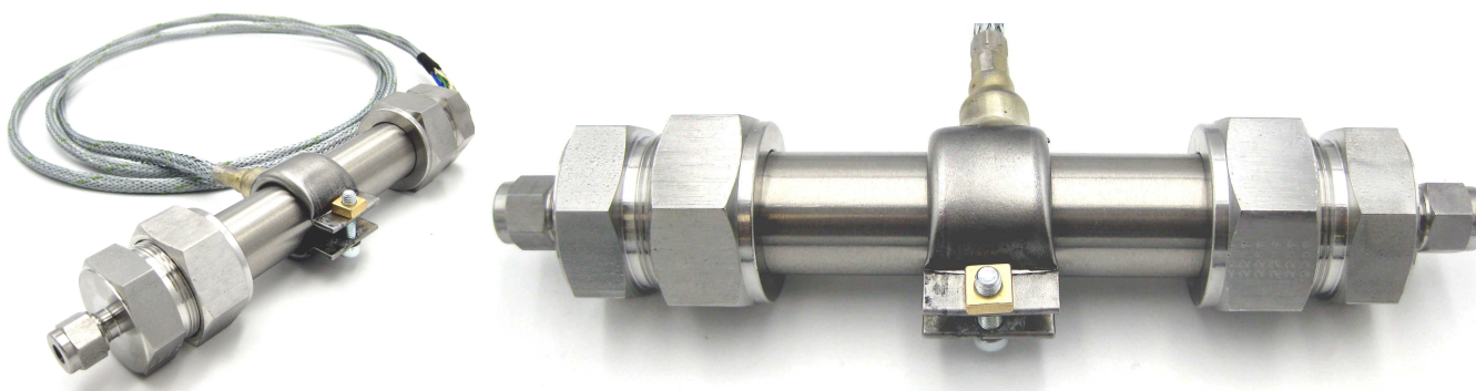
Figure 1: H 2 -burner version NEO305 with heating cable and optional adapter to 6mm compression fitting
