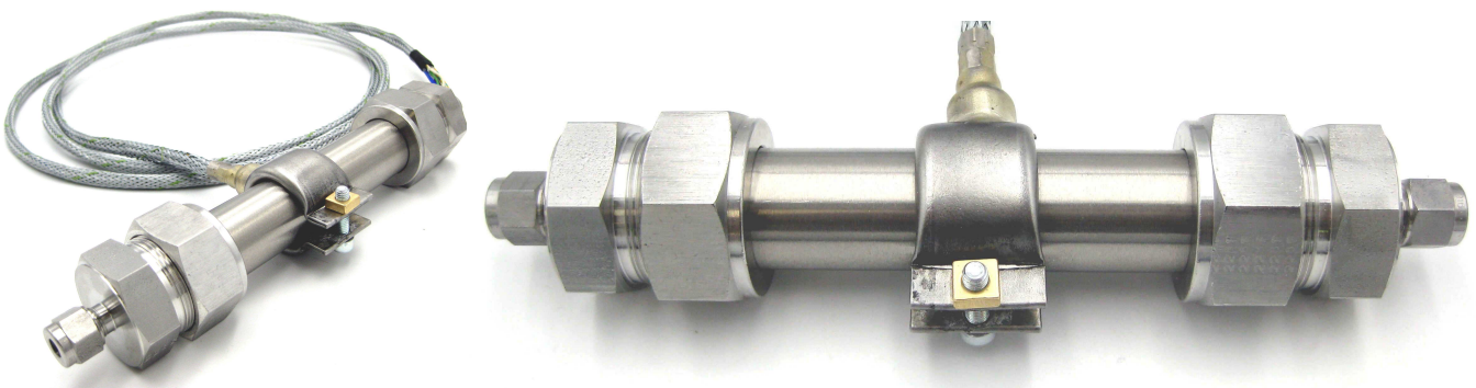
Figure 1: H 2 -burner version NEO305 with heating cable + optional adapter to 6.35mm compression fitting
