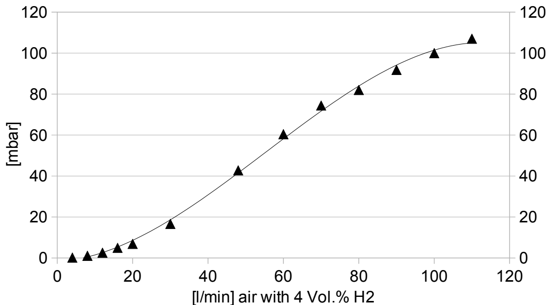
Figure 2: Back pressure at conversion of 4 vol.% H 2 in air, 20°C inlet temperature
