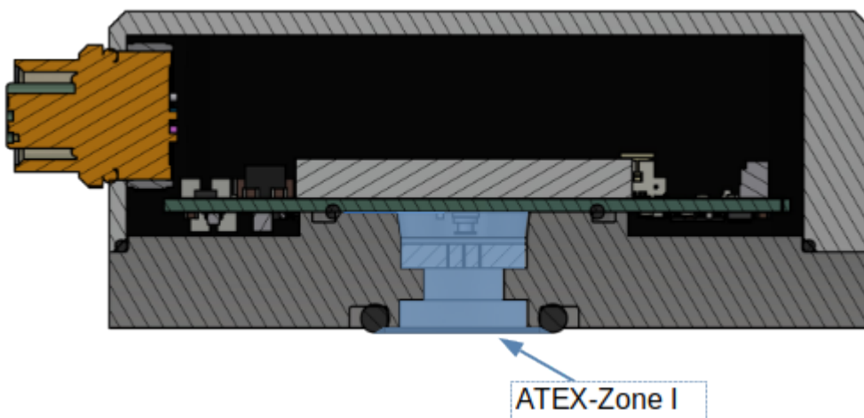
Figure 2b: ATEX Zone I
