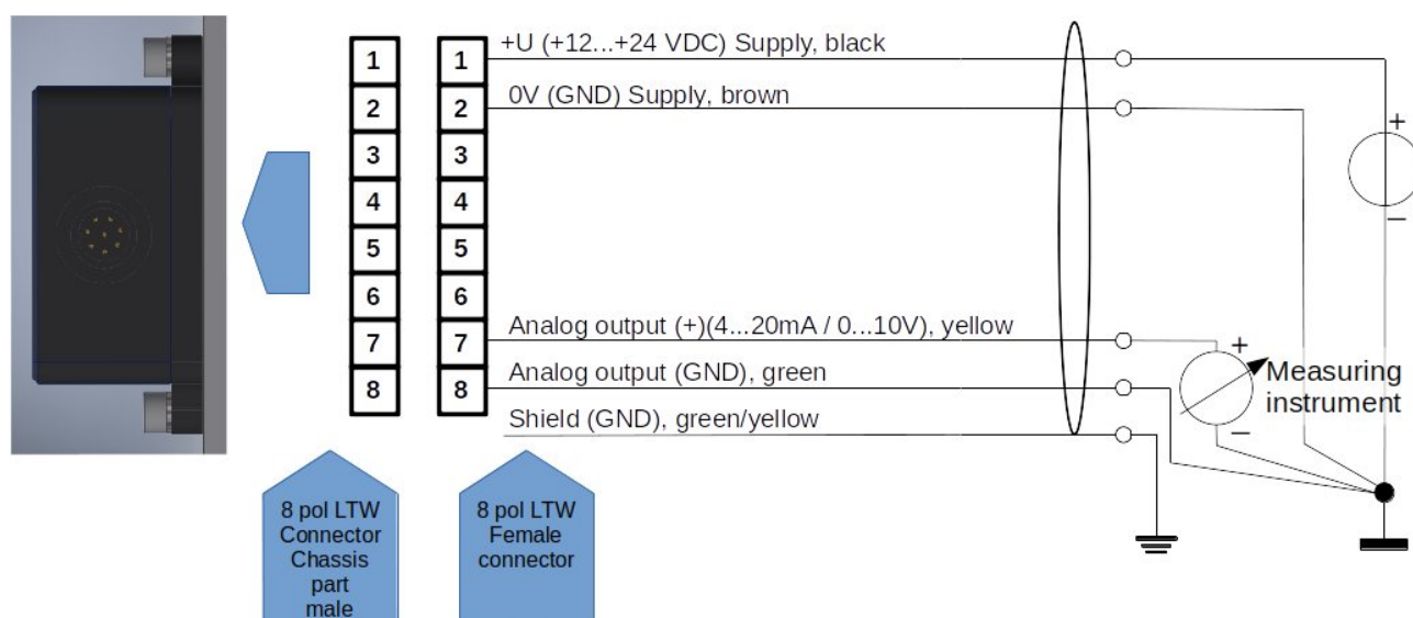
Figure 5: connection diagram
