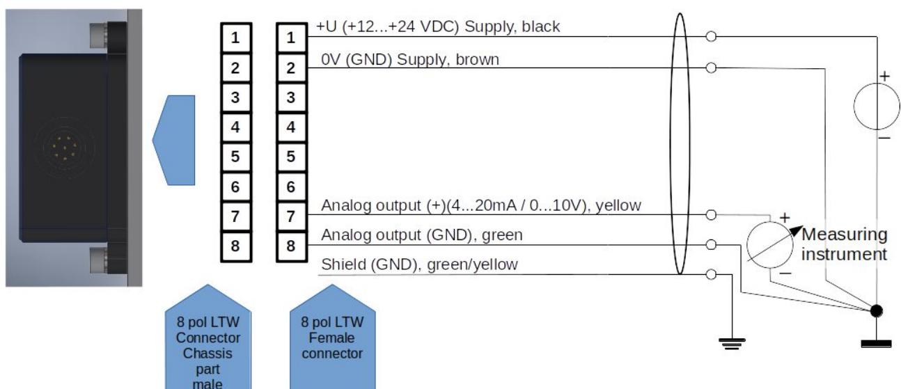
Figure 5: connection diagram
