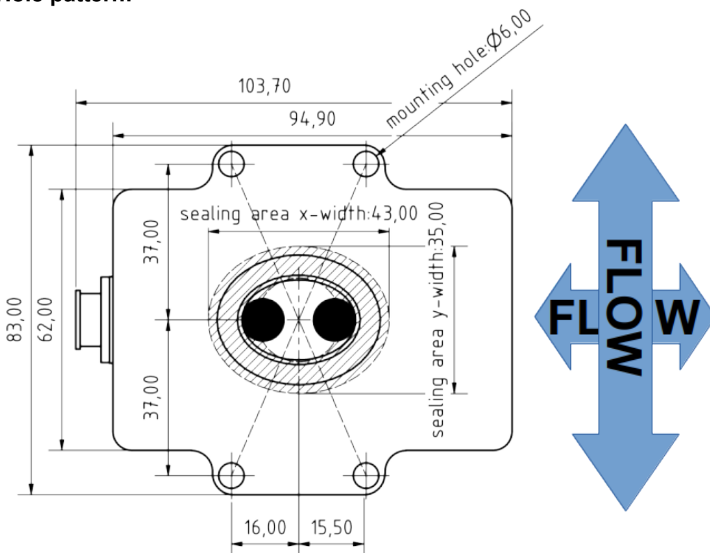
Figure 2b: NEO9XXHT-ATEX O-Ring sealing and sintered metal filter
